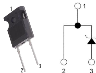
TO-247-2
